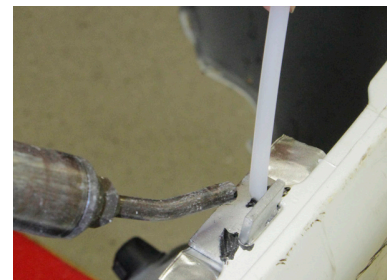
3. Weld around the die, approximate the original shape of the bumper.
